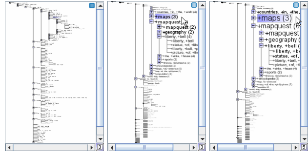
Figure 2: When the Fisheye Tree View is zoomed out, the vertex labels cannot be read (left). Applying different amounts of fisheye magnification re-enables readability for a focus vertex and its context (middle and right).
